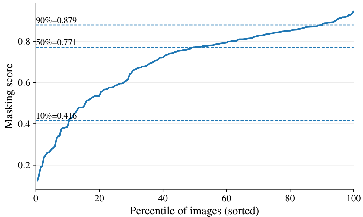
CIFAR-100
