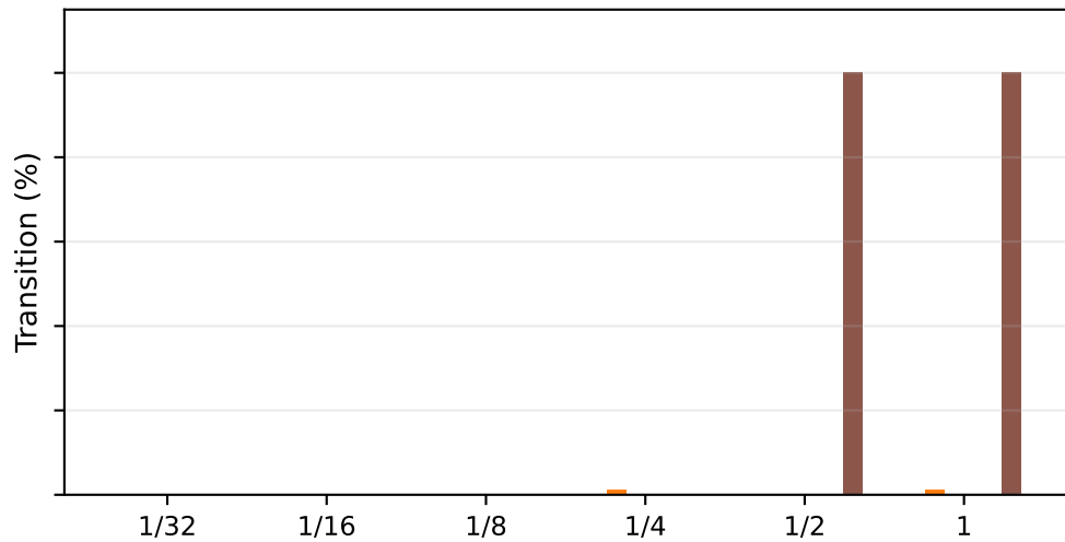
Global → Background
