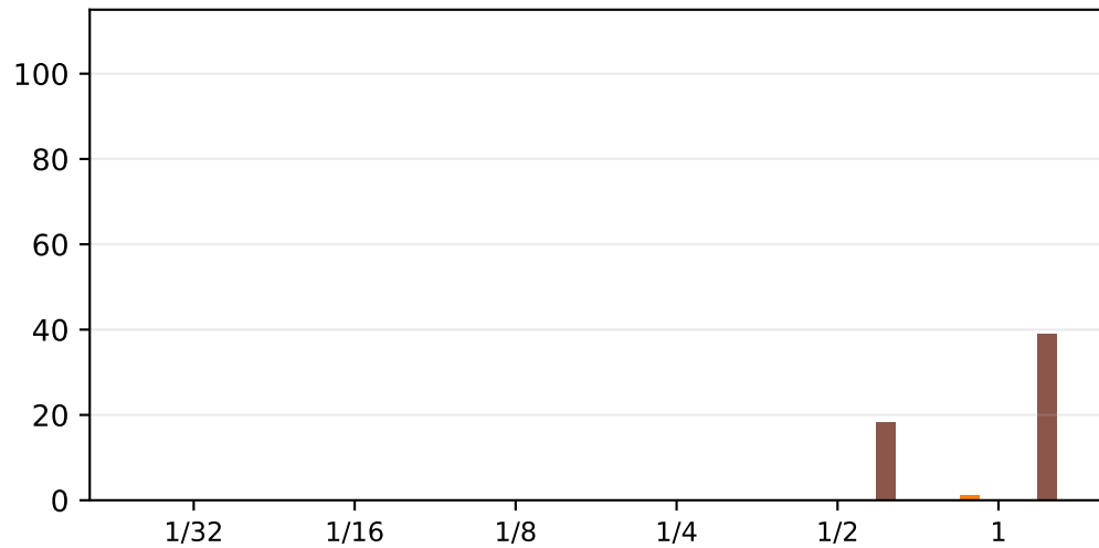
Global → Object
