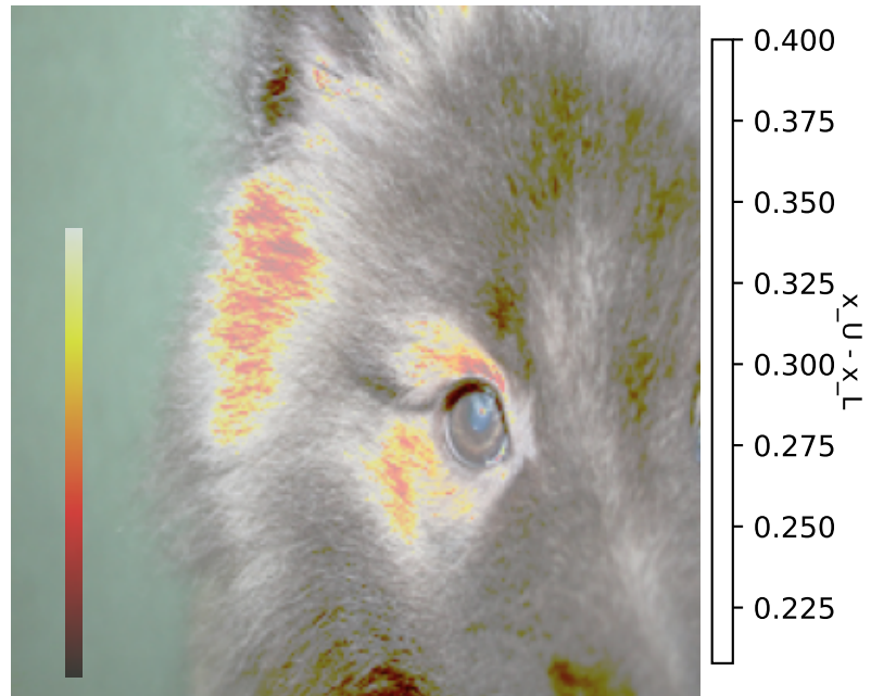
Bound Width Heatmap ( \epsilon = 0.2 )
