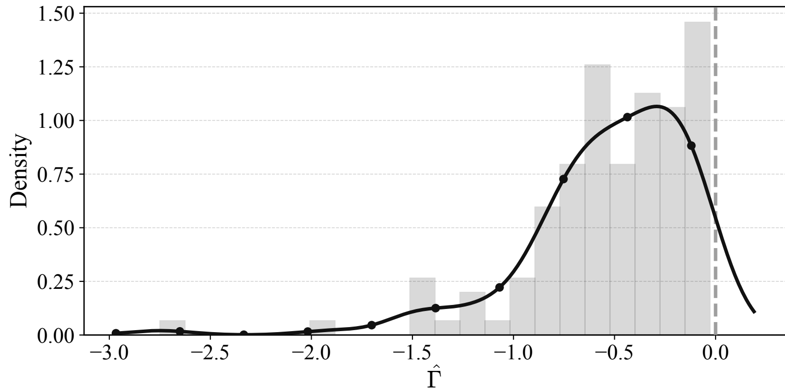
CIFAR-100
