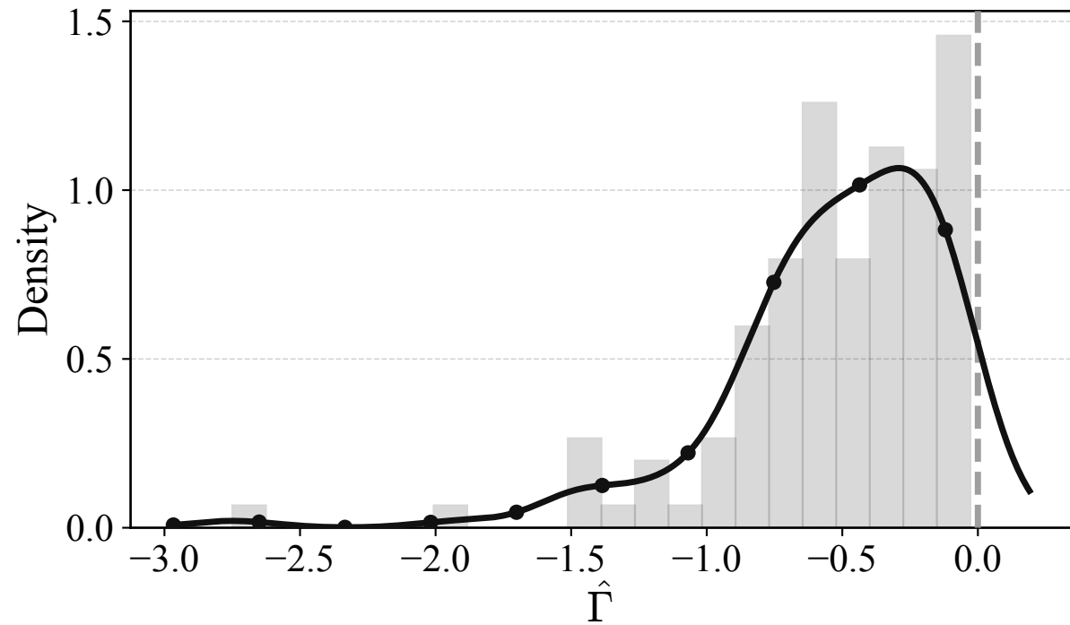
CIFAR-100
