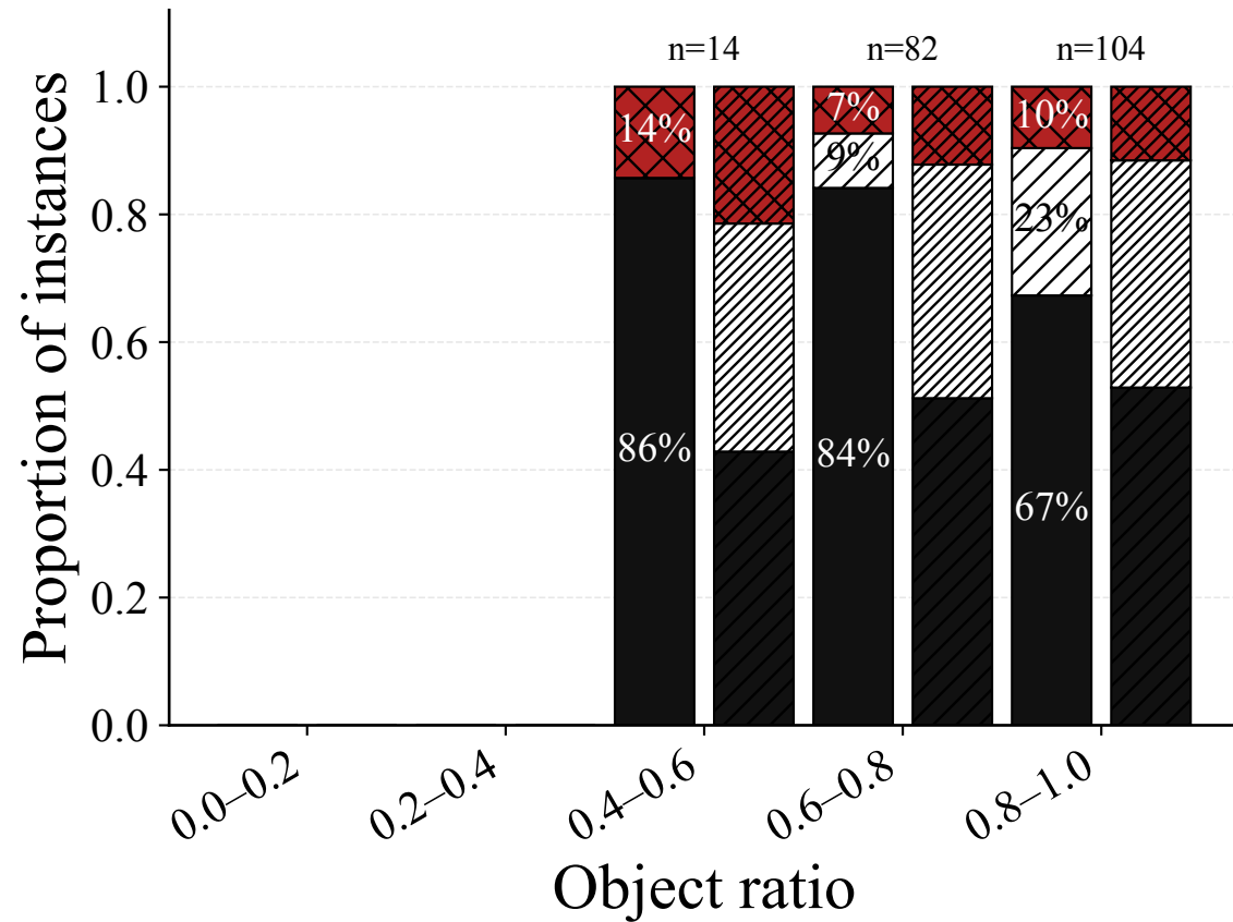
CIFAR-100
