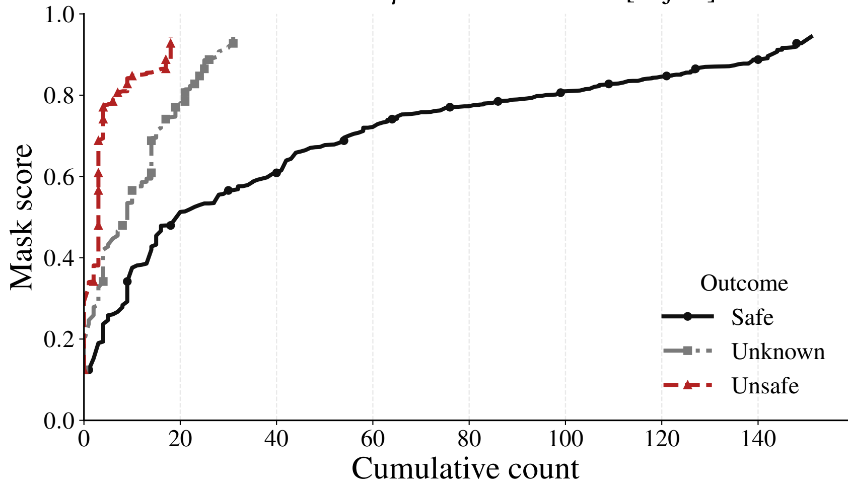
CIFAR-100: \alpha\beta -CROWN w/ CSI [object]
