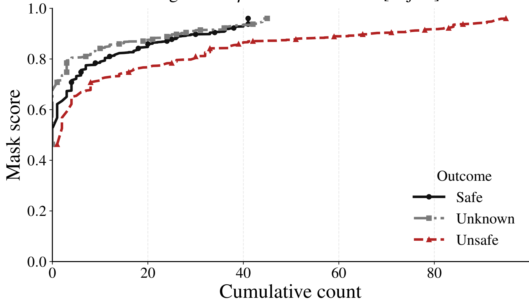
ImageNet: \alpha\beta -CROWN w/ CSI [object]
