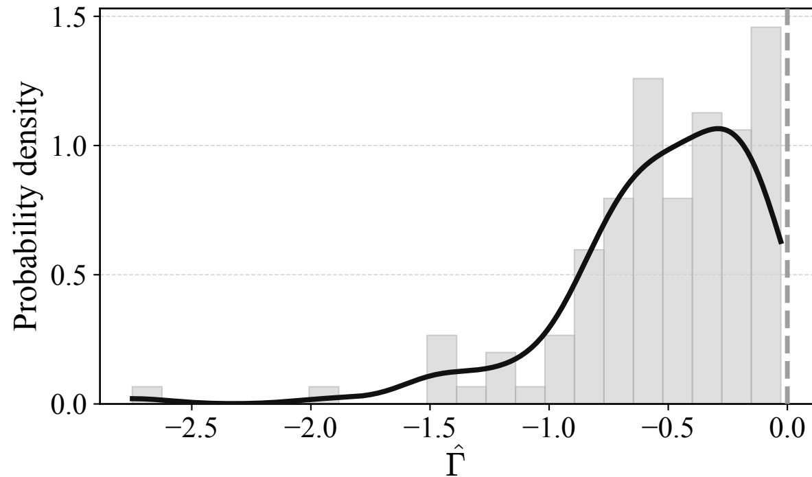
CIFAR-100
