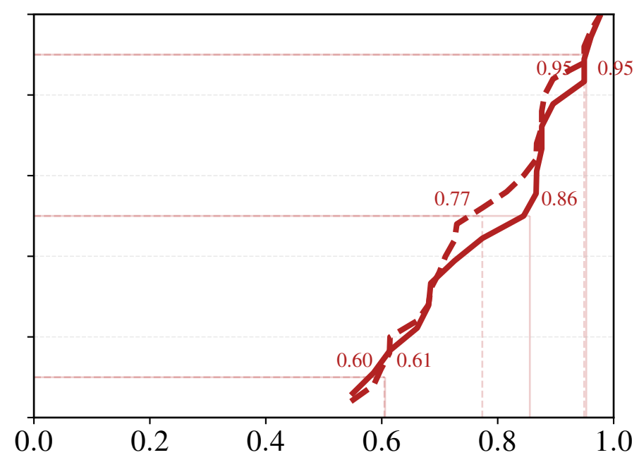
Unsafe — CIFAR-100
