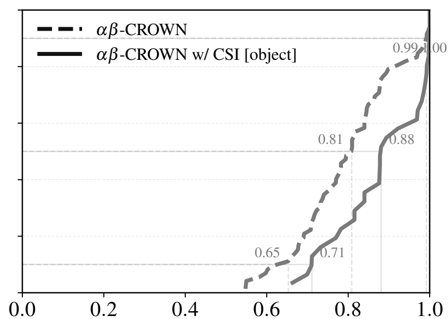
Unknown — CIFAR-100
