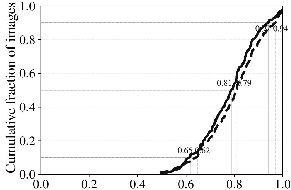
Safe — CIFAR-100
