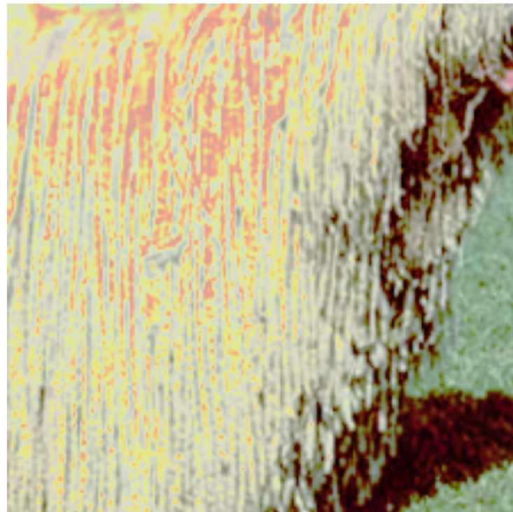
Bound Width Heatmap ( \epsilon=0.2 )
