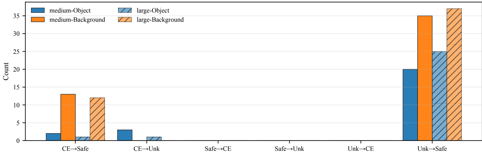
Global \rightarrow (Object/Background):status transitions in Medium vs Large models (CE/Safe/Unk) in cifar100
