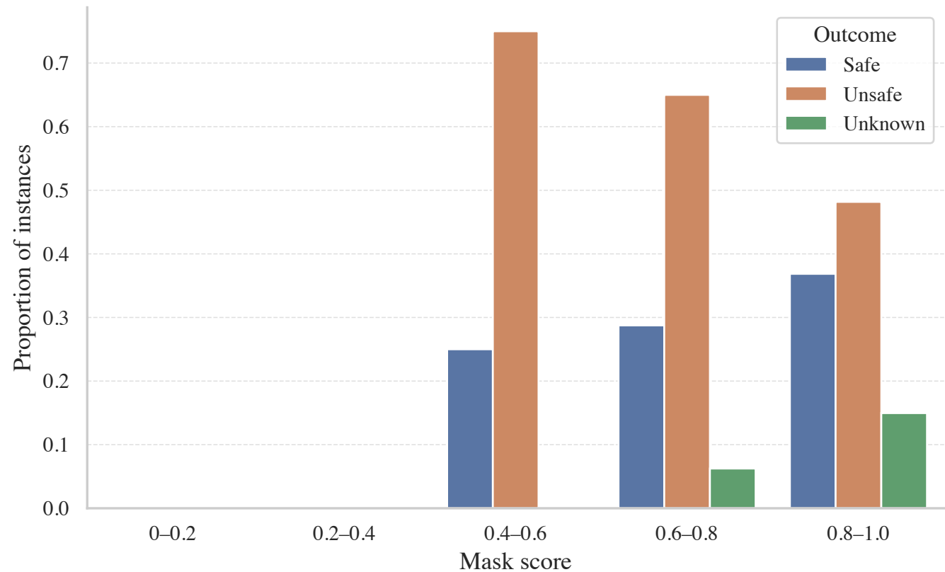
Verification outcome vs mask score (ImageNet)
