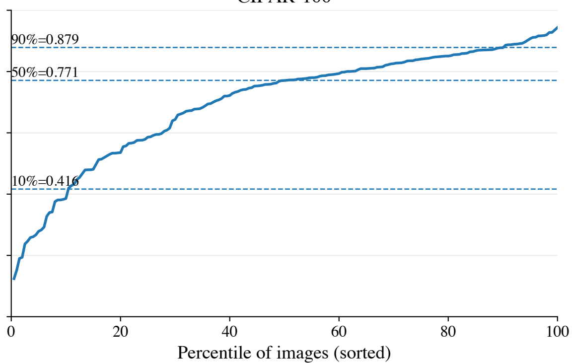
CIFAR-100
