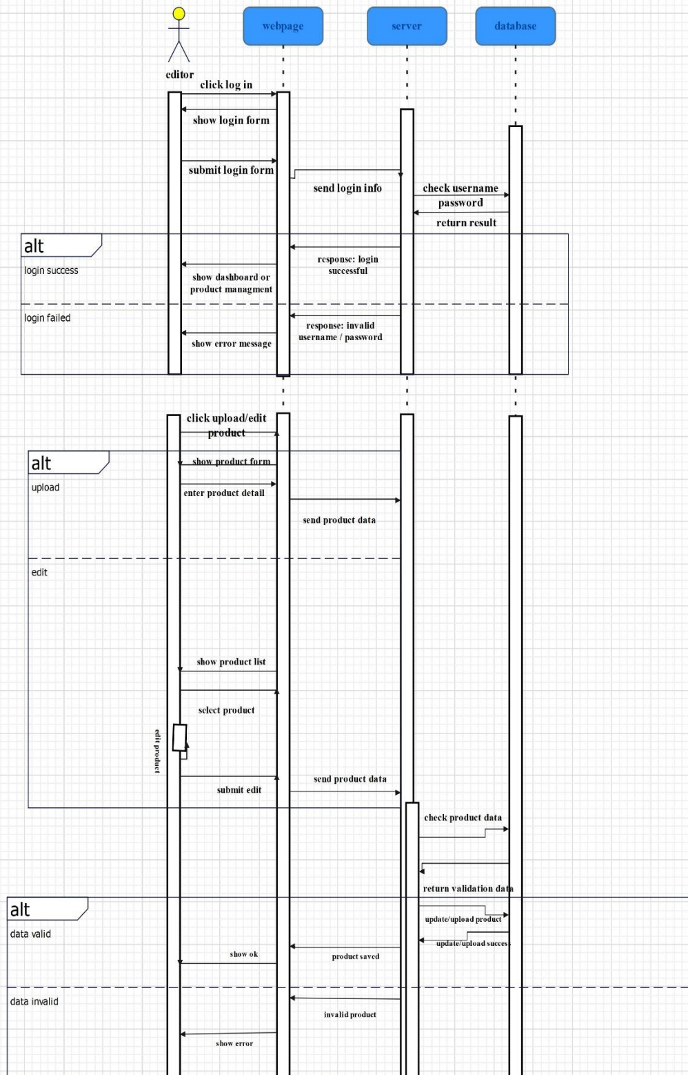
Sequence Diagram for upload/edit product
