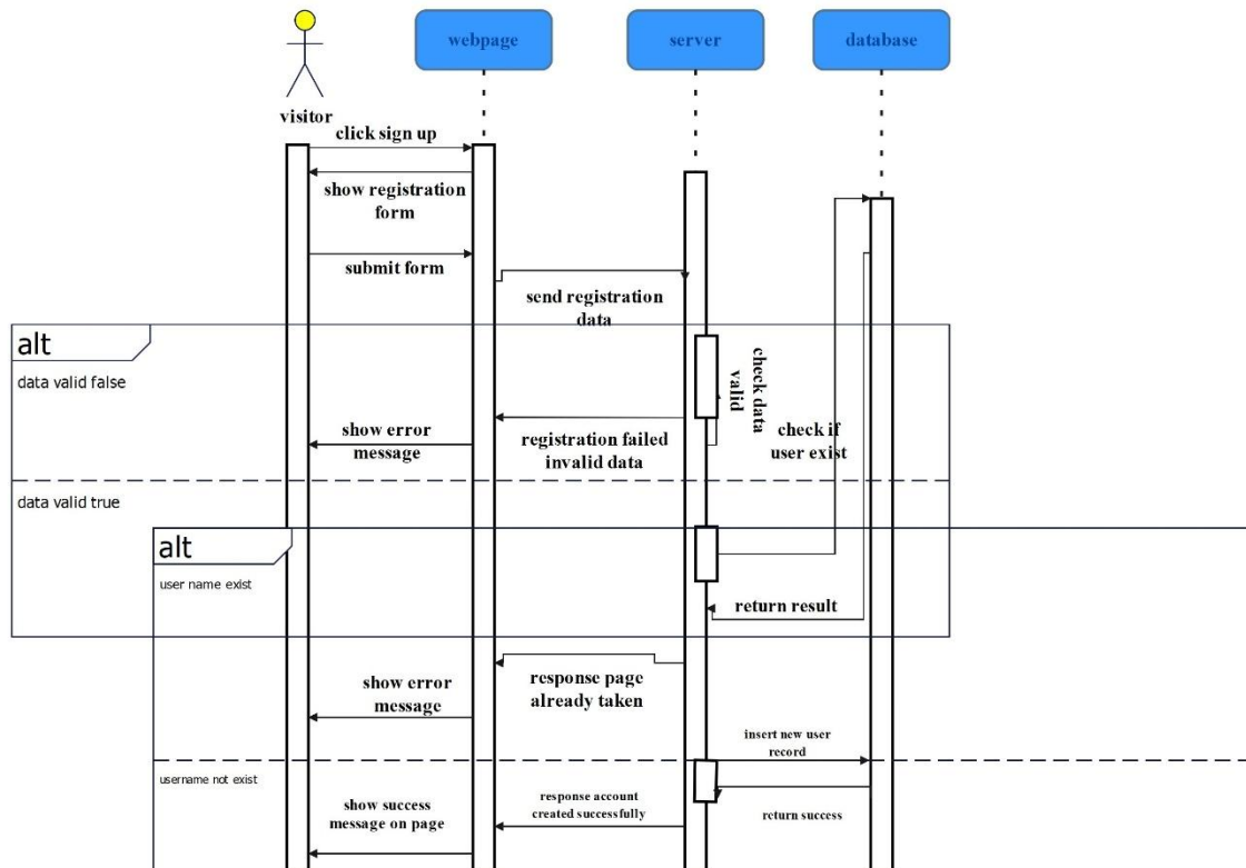
Sequence Diagram for create an account
