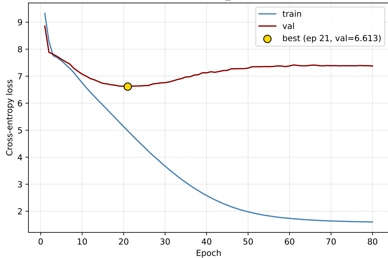
Phase 2 — Coptic→Syriac transformer (256d × 6L, peak_lr=3e-04)
