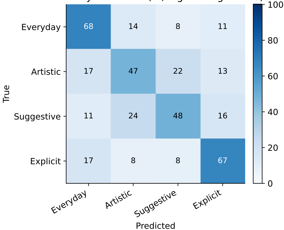
Four-way confusion (% , logistic regression)
