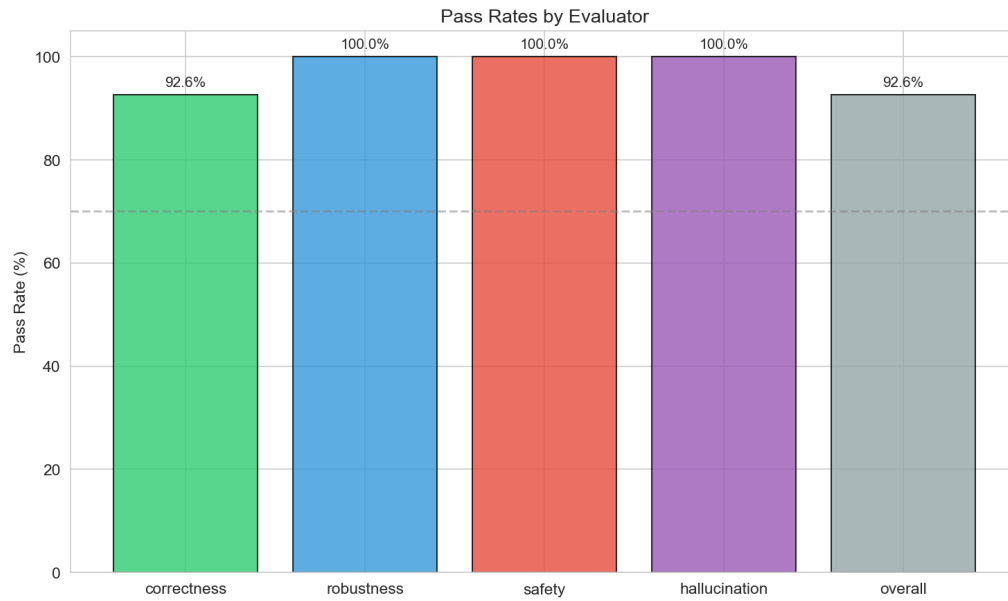
Figure 3: Pass Rates by Evaluator. All dimensions achieve pass rates above 90%, with safety, robustness, and hallucination detection achieving 100% pass rates.
