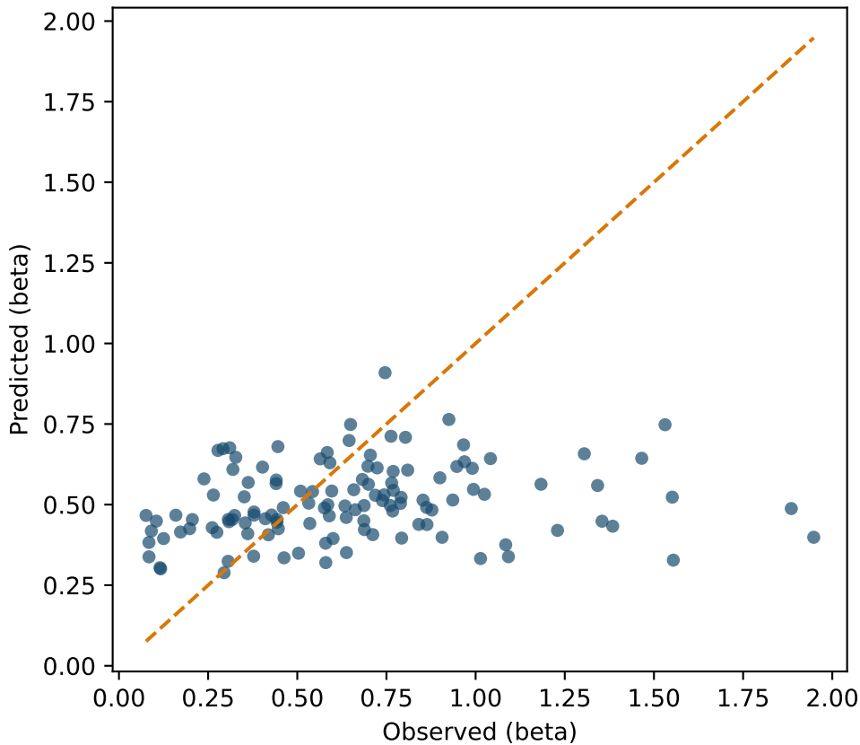
Locked test: predicted versus observed (n=123)
