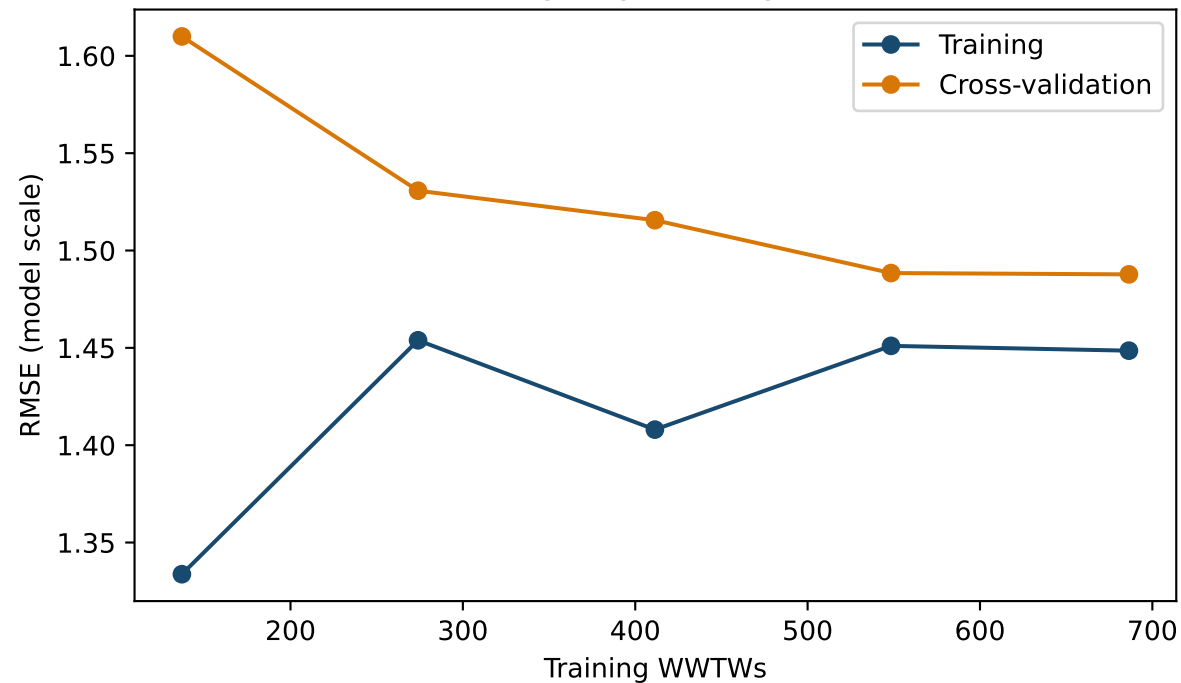
Training-only learning curve
