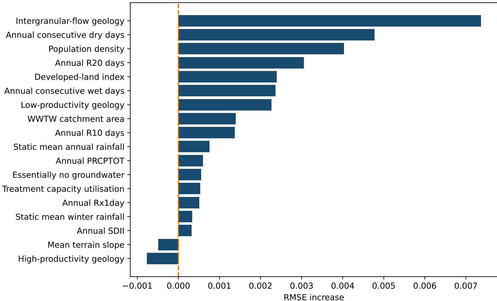
Locked-test permutation importance
