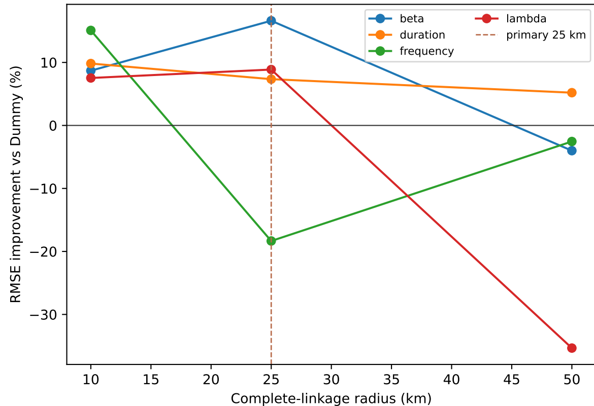
Regional radius sensitivity (fixed Ridge benchmark)
