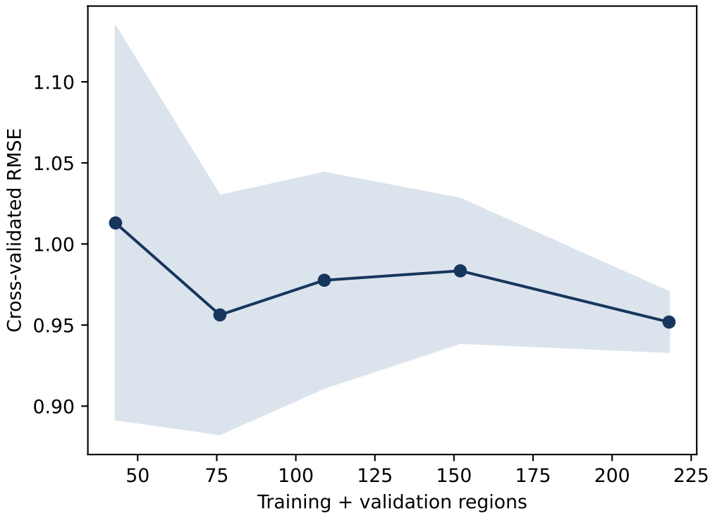
Pooled mean duration: learning curve
