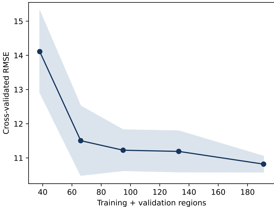
Regional lambda: learning curve
