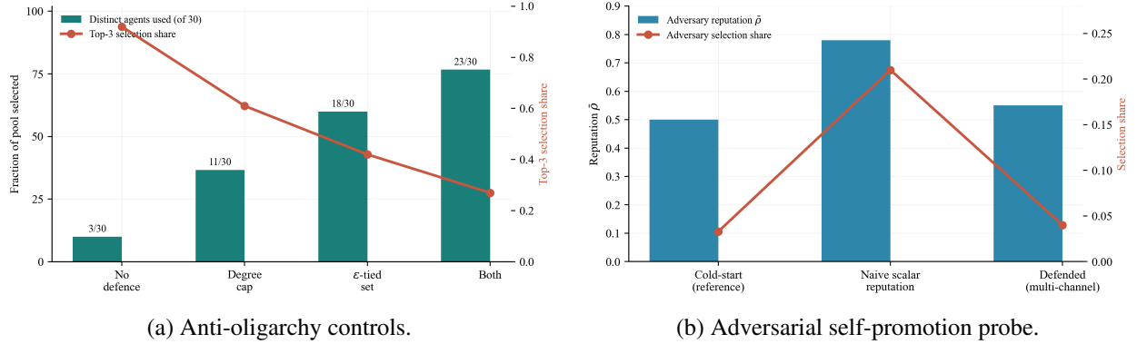
Figure 10: Robustness diagnostics. Exploration and the degree cap together prevent selection collapse; credibility-weighted updates limit adversarial reputation inflation.
