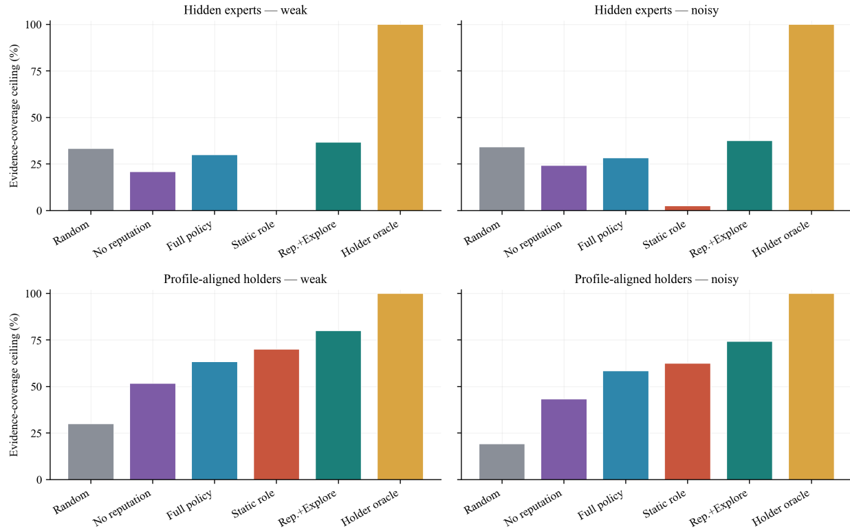
Figure 5: Live private-evidence coverage ceiling. Each bar is the fraction of rows whose selected team holds all required evidence. REP+EXPLORE is the strongest learned policy when holders are profile-aligned (bottom); when experts are hidden (top), every learned policy sits near RANDOM.
