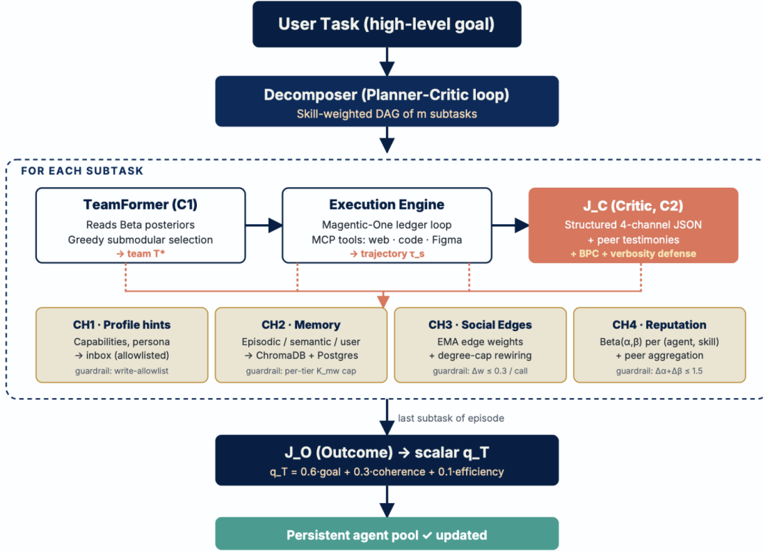
Figure 1: The CONOID episode loop. A decomposer turns the user task into a skill-weighted DAG of subtasks through a planner–critic loop. For each subtask, the team former (C1) reads the agents’ per-skill Beta posteriors and selects a team by greedy submodular optimization; the team executes inside a Magentic-One-style ledger loop with optional tools and returns a trajectory. A subtask critic J_C (C2) then emits one structured JSON object that updates four channels at once — profile hints, tiered memory, social edges, and per-skill reputation — under per-channel guardrails and the bias defenses of Section 3.3. After the subtask tree finishes, an outcome judge J_O scores the episode and the updated pool becomes the prior for the next task.
