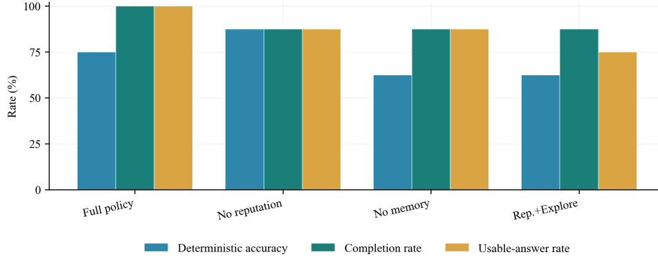
Figure 8: Live hard-control pilot (32 rows). The no-reputation control has the highest raw accuracy; the full system’s advantage is reliability — it always completes and always returns a usable answer.
