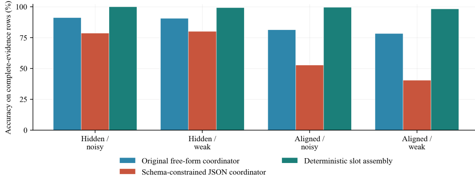
Figure 7: Coordinator replay on complete-evidence rows (1,440 calls). Schema enforcement removes parse errors but loses facts; deterministic slot assembly recovers them.
