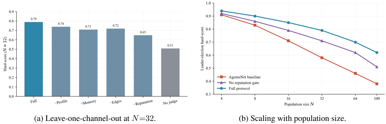
Figure 9: Internal validation on the coordination substrate. Removing any channel lowers hard-score; the reputation gate’s contribution grows with population size.
