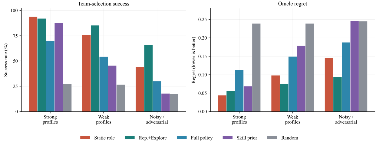
Figure 3: Profile-sensitivity benchmark (691,200 rows). Static role assignment is strongest when profiles are reliable; the reputation-plus-exploration policy is strongest when profiles are weak or adversarially noisy. Bars are means over 40 seeds.
