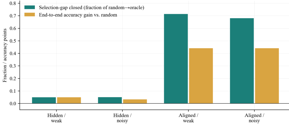
Figure 6: Distance from random to the holder oracle. REP+EXPLORE recovers most of the evidence-selection gap and yields a large end-to-end accuracy gain only when evidence is profile-aligned; hidden-expert discovery stays near chance.
