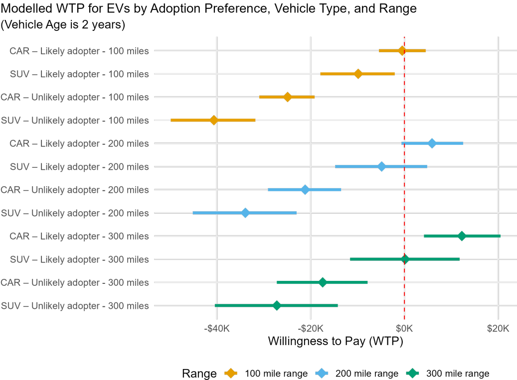
Figure 2: Modelled WTP for used BEVs by adoption preference, vehicle type, and driving range (vehicle age fixed at 2 years). Points show point estimates; horizontal bars show 95% simulation confidence intervals.
