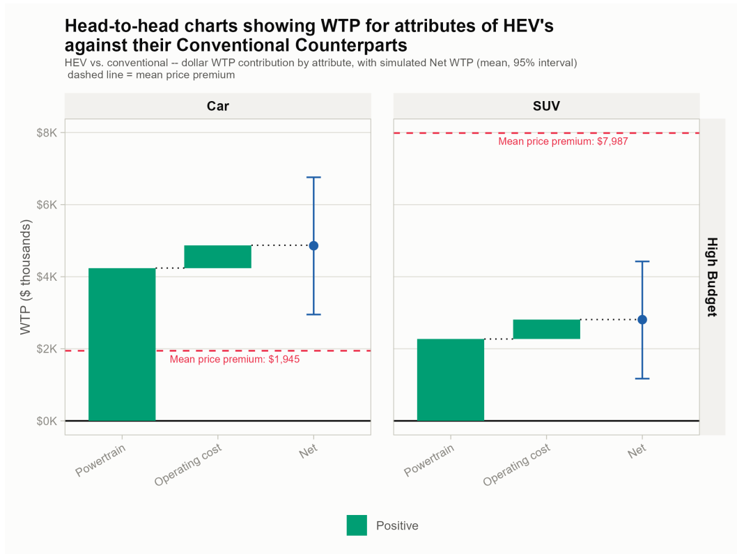
Figure 4: Willingness-to-pay decomposition (powertrain and operating cost) for real, currently marketed HEV vehicles relative to each vehicle's closest conventional counterpart, by vehicle segment and budget tier. The blue point/error bar is simulated Net WTP (mean, 95% interval); the dashed red line is the observed mean real-market price premium at approximately three years of age. No matched HEV pair meeting the sample-size threshold was available in either low-budget segment.
