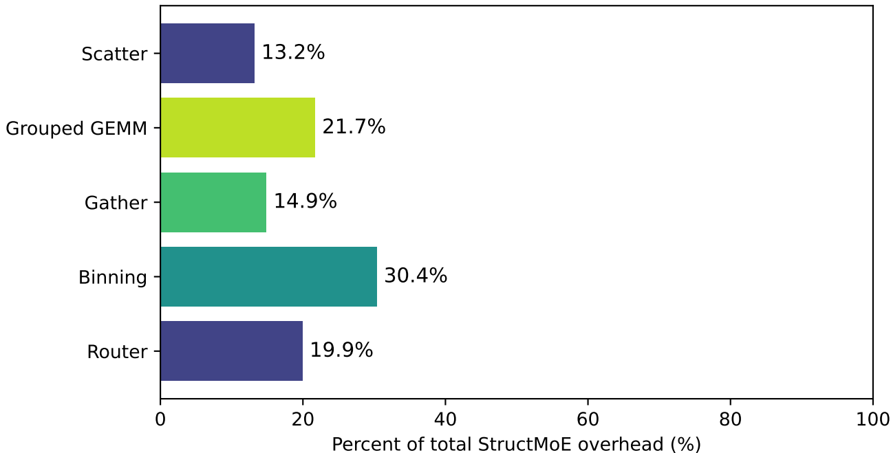
Breakdown of StructMoE Overhead (Relative %)
