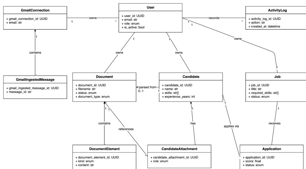
Figure 4.5: Class Diagram
