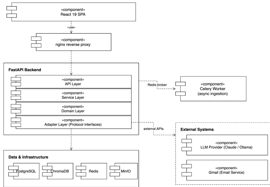
Figure 4.7: Component Diagram
