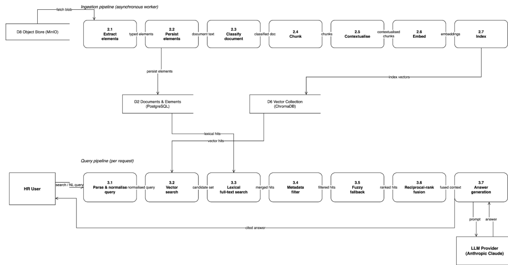
Figure 4.4: DFD Level 2
