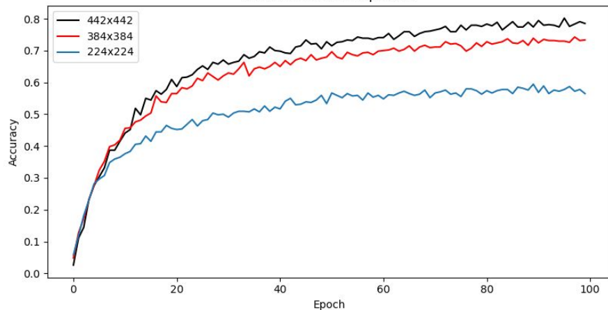
Validation Acc. Comparison
