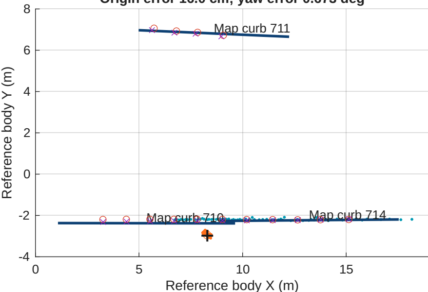
Frame 932: 15 confirmed curbs + 1 historical pole Origin error 16.0 cm; yaw error 0.673 deg
