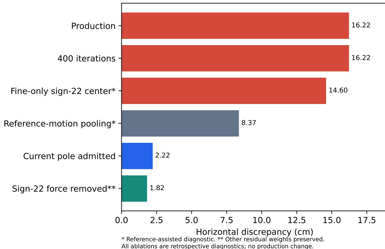
Fixed-frame counterfactuals
