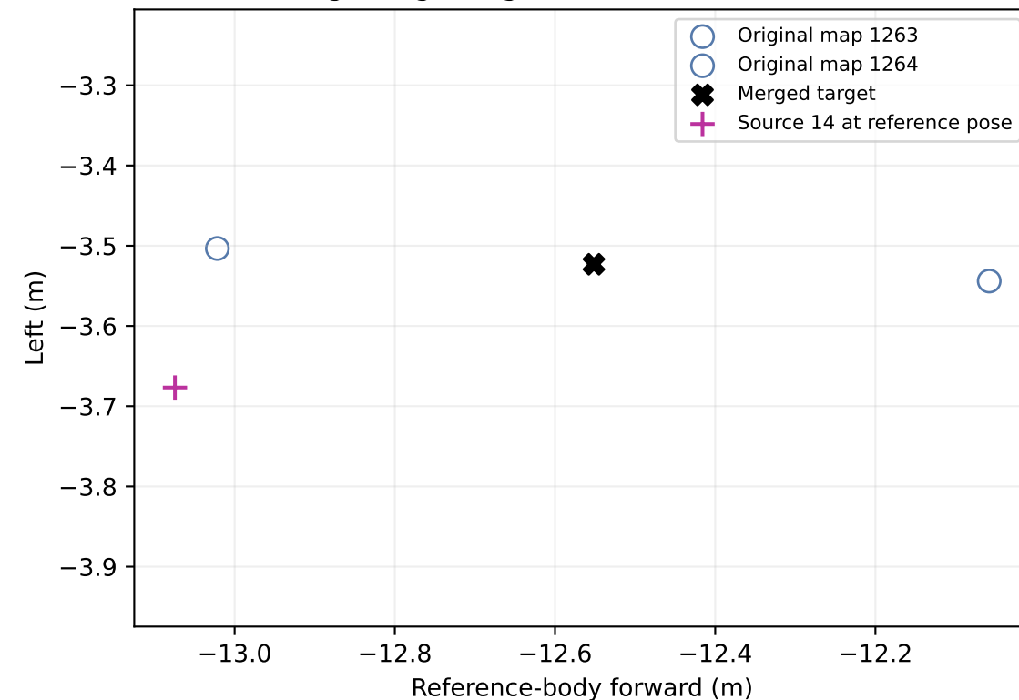
Merged sign target is 54.5 cm from source
