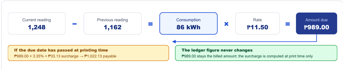
Figure 7.1 — How a bill is computed. Surcharge is never written into the bill record. It is recalculated whenever the receipt is printed, so a receipt always shows what is owed today while the ledger keeps what was originally billed.
