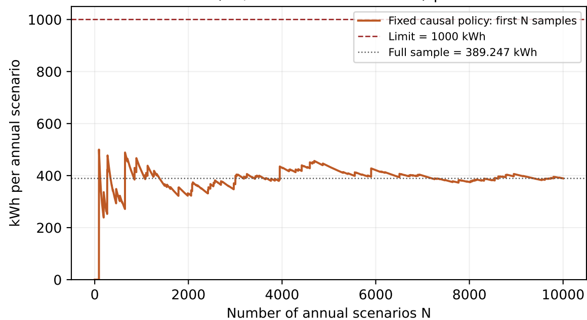
Validation (10,000 annual scenarios) | CVaR 0.95
