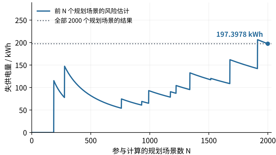
CVaR 0.95 | 约束上限 1000 kWh
