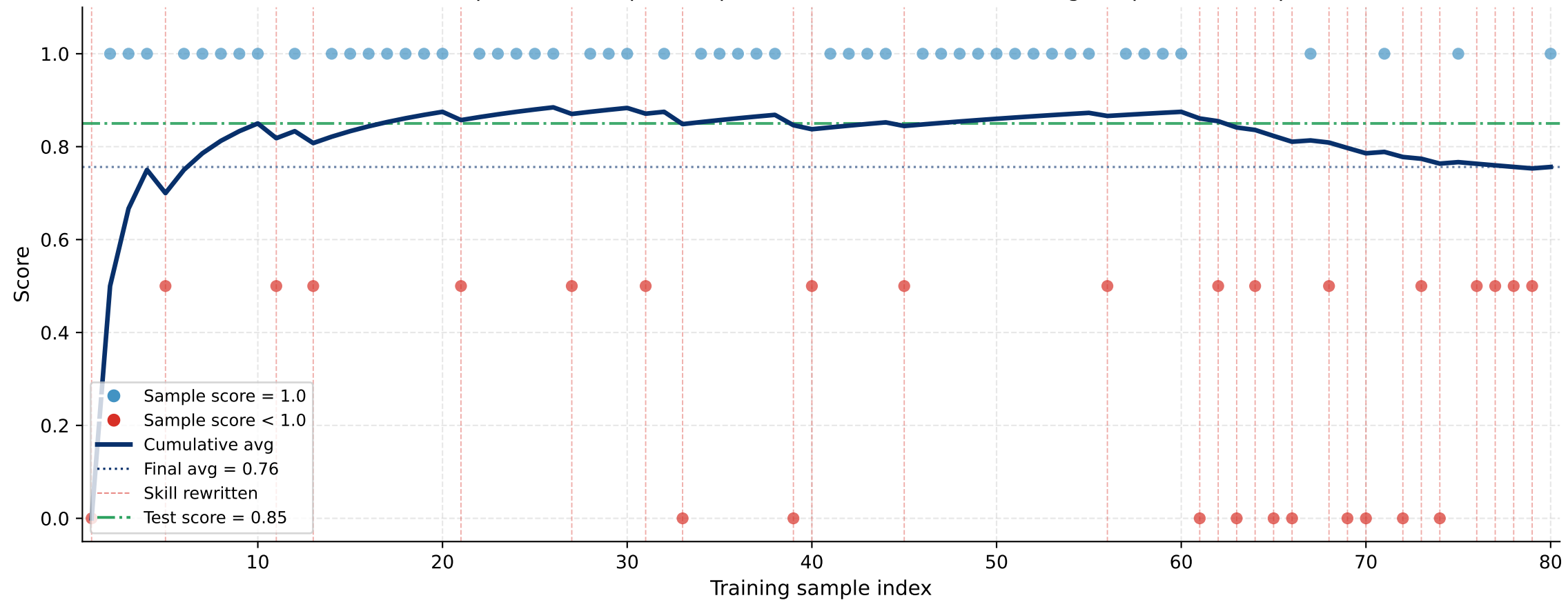
ATL — Online specialization: per-sample score and cumulative average (1 pass, 80 samples)
