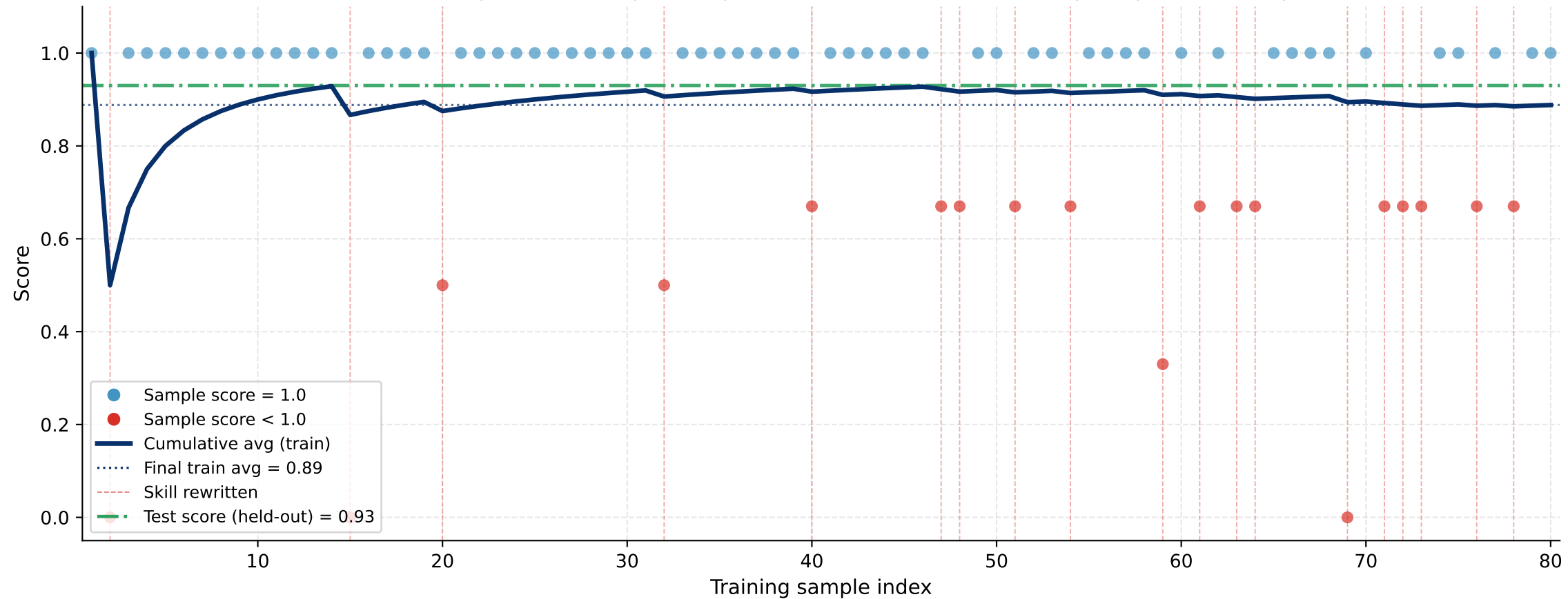
EMF — Online specialization: per-sample score and cumulative average (1 pass, 80 samples)
