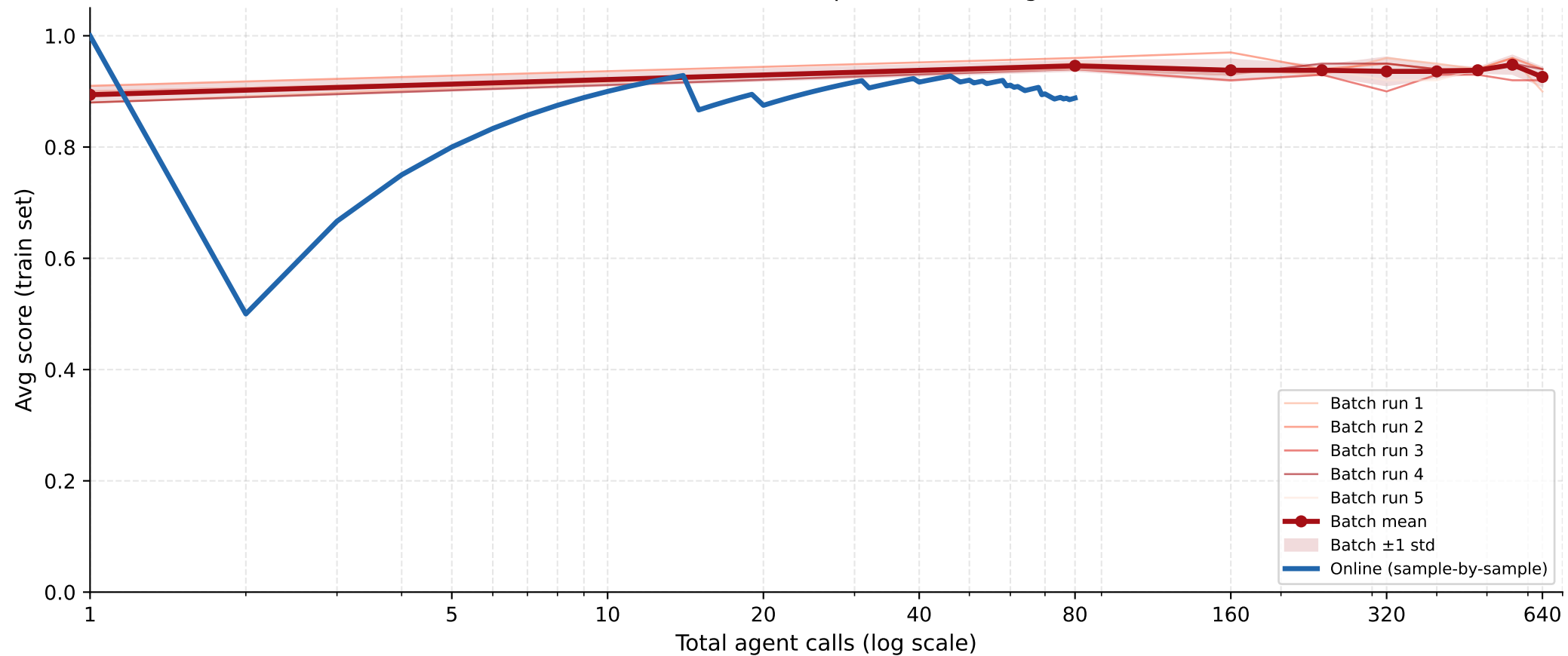
EMF — Online vs Batch specialization (log scale)
