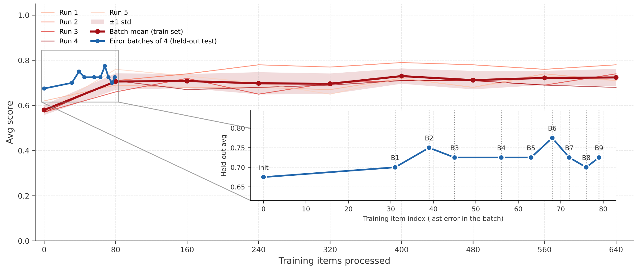
ATL (model transformations) :batch iterations vs. error batches
