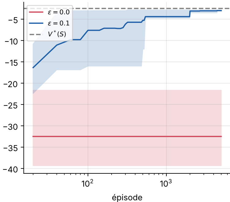
V^{\pi_t}(S) , initialisation pessimiste Q_0 = -100
