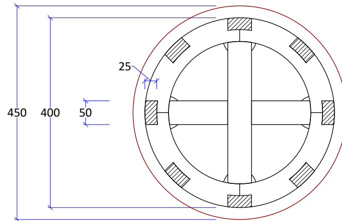
SECTION TOP VIEW
