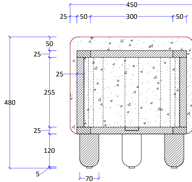
SECTION FRONT VIEW
