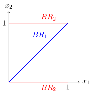
Figure 4.1: Continuous Matching Pennies: best responses never intersect.
