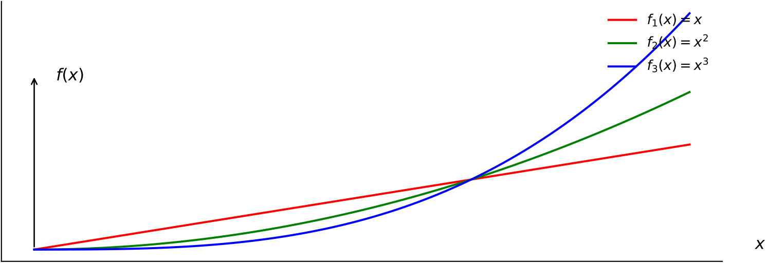
Example 1: Polynomial ( h_m = x^m )
