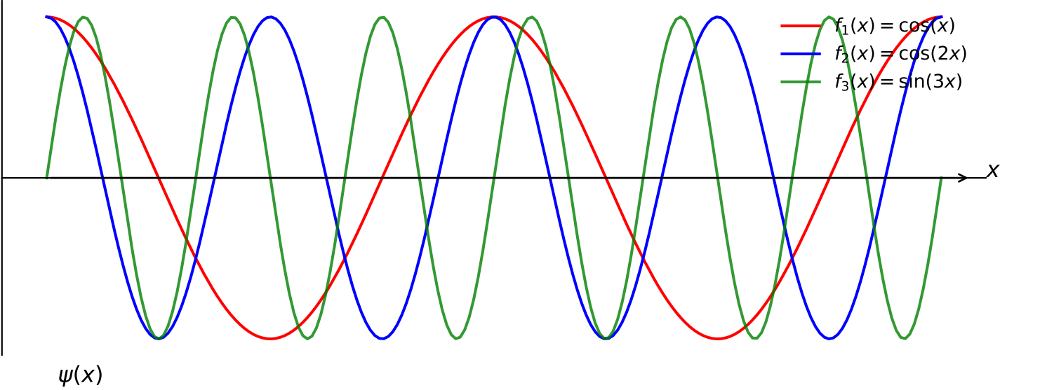
Example 2: Fourier
