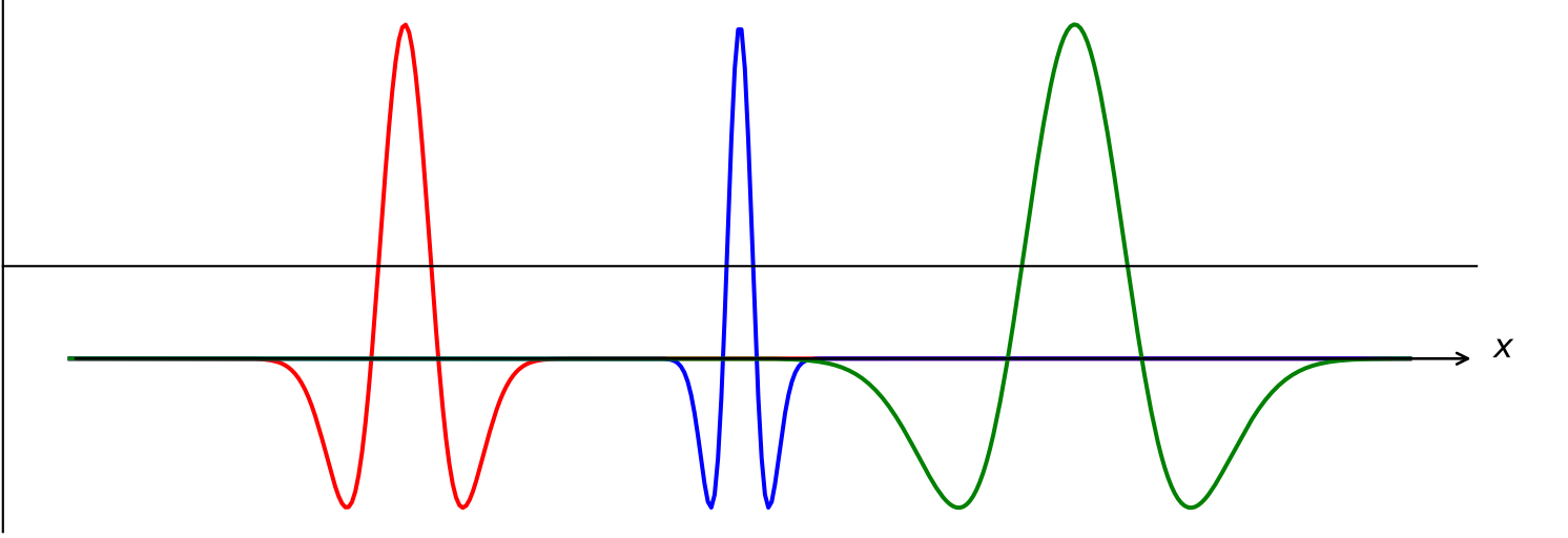
Example 3: Wavelets
