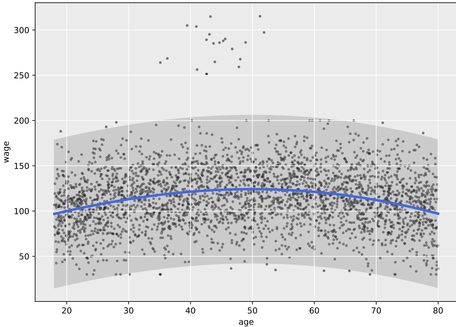
4-degree Polynomial
