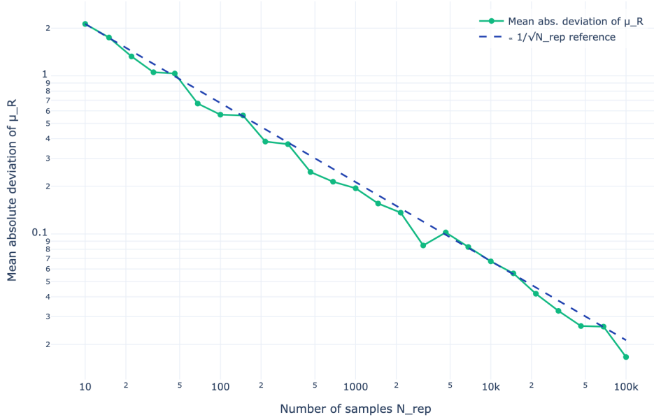
Figure 6: Convergence of the exact steady-state sampler’s empirical moments to the analytical steady-state values as a function of the number of samples N_{\text{rep}} . The error (shown as mean absolute deviation) decays as 1/\sqrt{N_{\text{rep}}} , as expected from the Central Limit Theorem.
