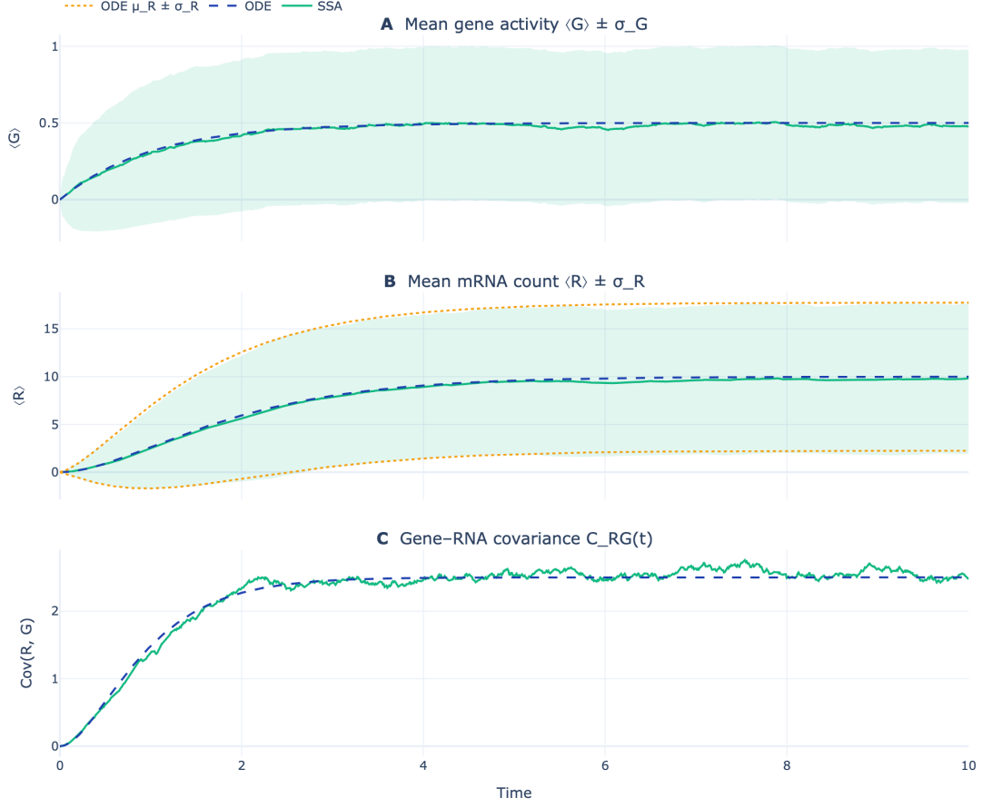
Figure 3: SSA ensemble averages (green, with the empirical \pm \sigma fluctuation bands shaded) and the deterministic ODE solutions (dashed blue) at the reference parameters from (g_0, r_0) = (0, 0) , with N_{\text{rep}} = 1000 . In the mRNA panel the analytical spread from the moment ODEs, \mu_R \pm \sigma_R , is drawn as amber dotted lines on top of the SSA band.
