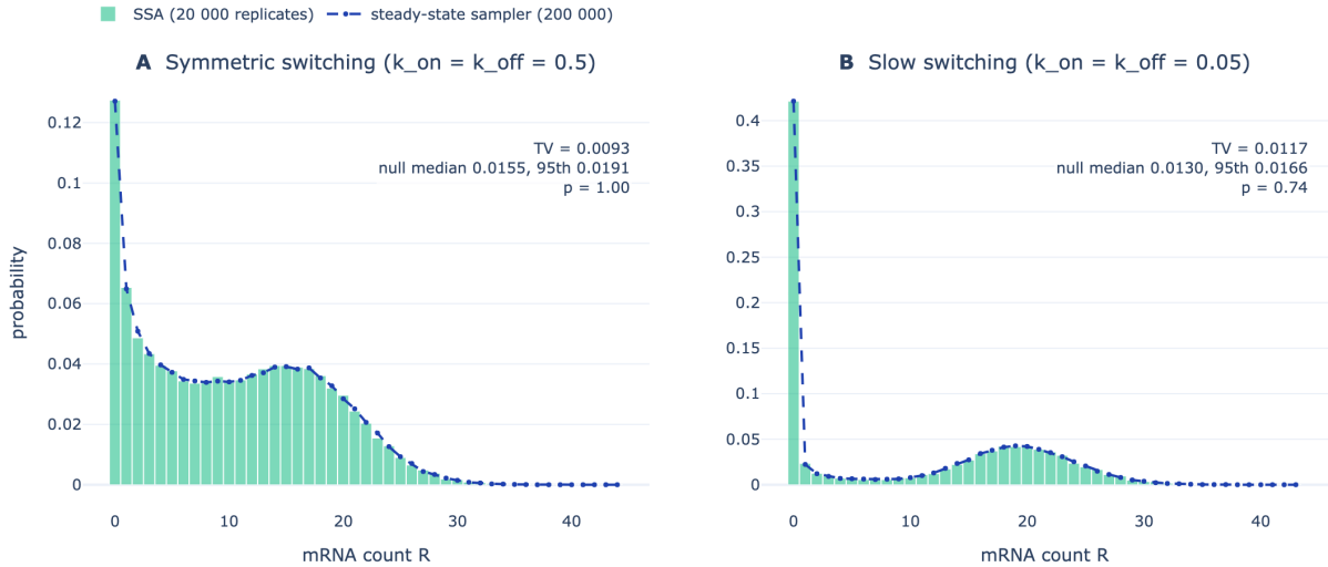
Figure 7: Edge 3 as a distributional test: the stationary mRNA distribution from 20 000 independent SSA trajectories (green bars, read at one late time per replicate) against 2 \times 10^5 draws from the steady-state sampler (dashed blue). Left: the symmetric reference regime. Right: slow switching ( k_{\text{on}} = k_{\text{off}} = 0.05 ), where the exact law is bimodal, with modes at R = 0 and near R = k_{\text{syn}}/k_{\text{deg}} = 20 and a trough at the mean \mu_R = 10 . Each panel gives the observed total-variation distance with the median and 95th percentile of the resimulated null band and the one-sided p -value.
