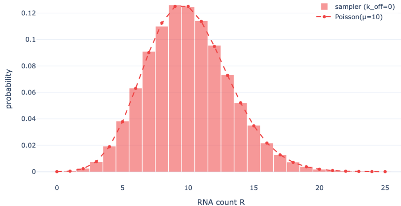
Figure 8: Edge case k_{\text{off}} = 0 (permanently active gene). The sampled steady-state mRNA distribution matches the analytic Poisson PMF with mean k_{\text{syn}}/k_{\text{deg}} = 10 (Fano factor \approx 1 ), the exact limit the telegraph model must reduce to when the gene never switches off.
