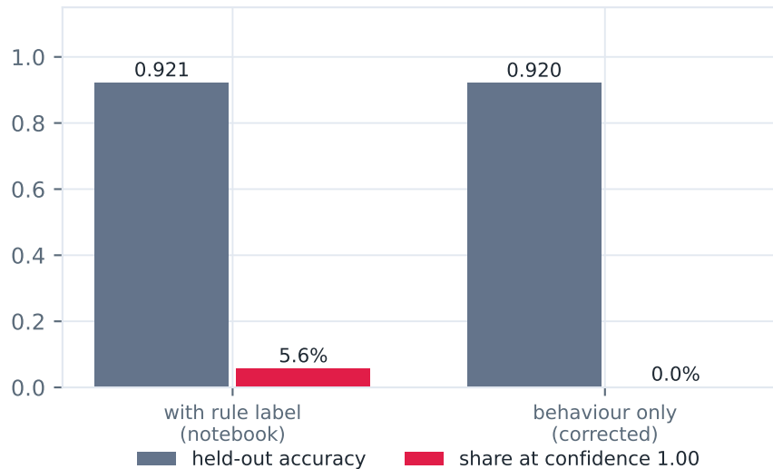
Defect 1 — leakage inflates certainty, not accuracy
