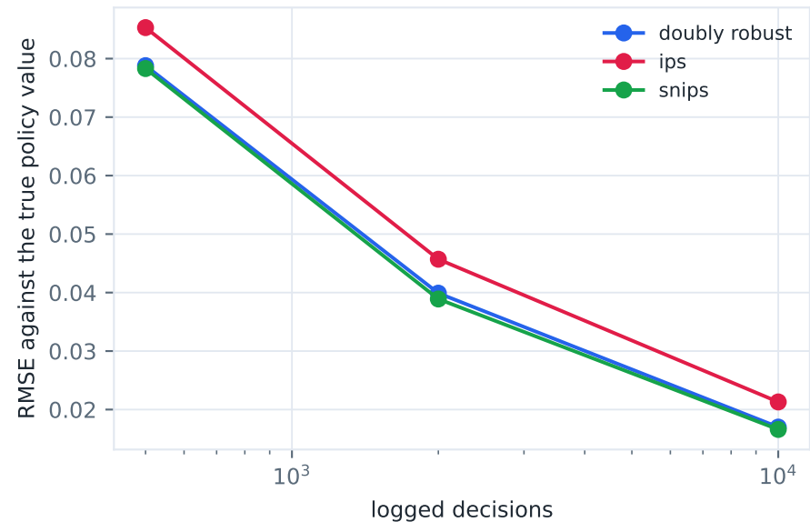
The estimate sharpens as the log grows
