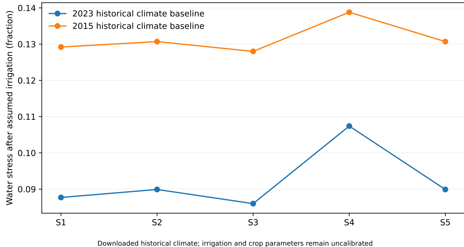
Scenario stress with downloaded Open-Meteo climate
