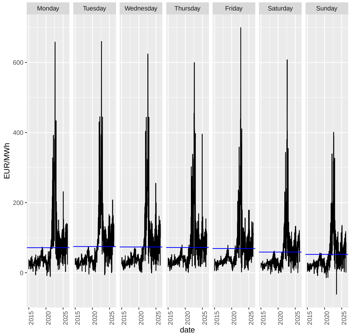
DK1 prices by day of week
