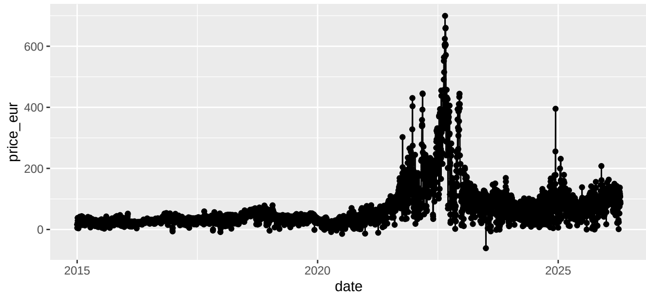
DK1 price – time plot, ACF, PACF
