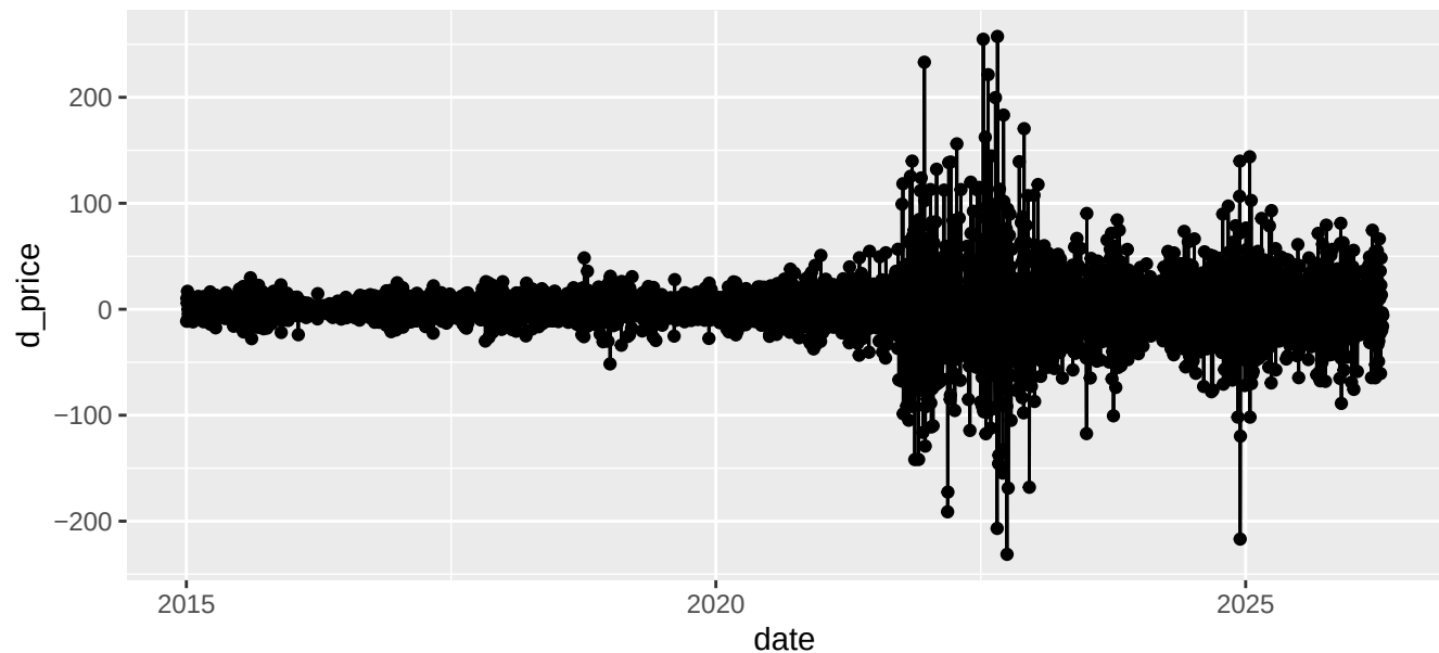
First-differenced DK1 price – time plot, ACF, PACF
