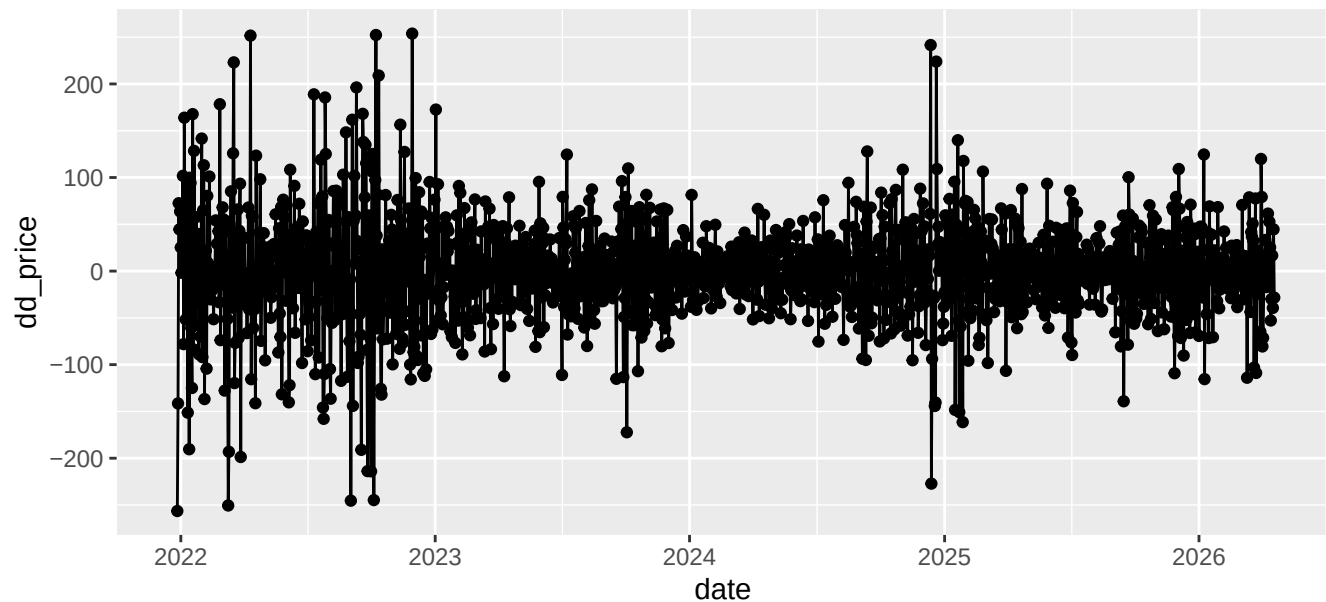
Seasonally + first differenced post-break d_price
