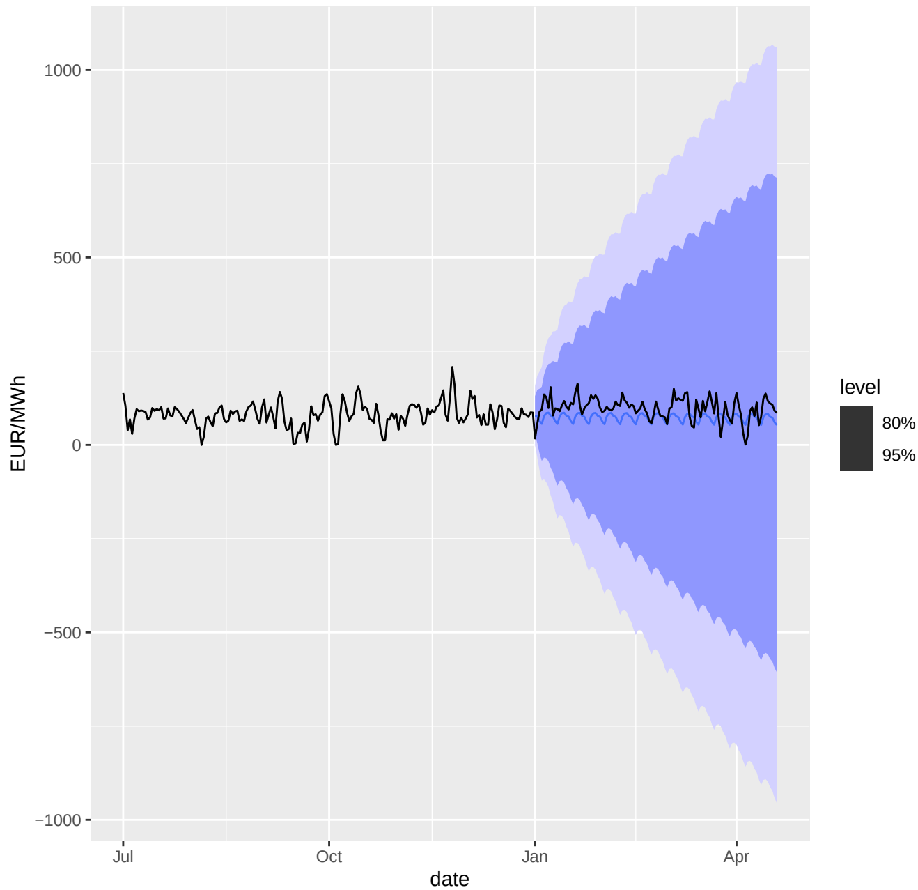
Manual ARIMA (airline) forecast vs actual
