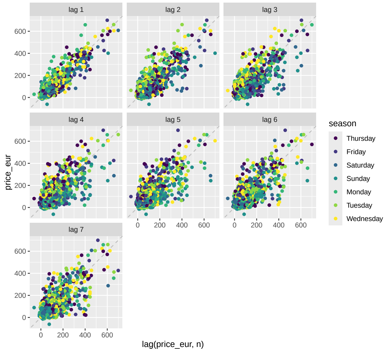
Lag plot of DK1 prices, lags 1–7
