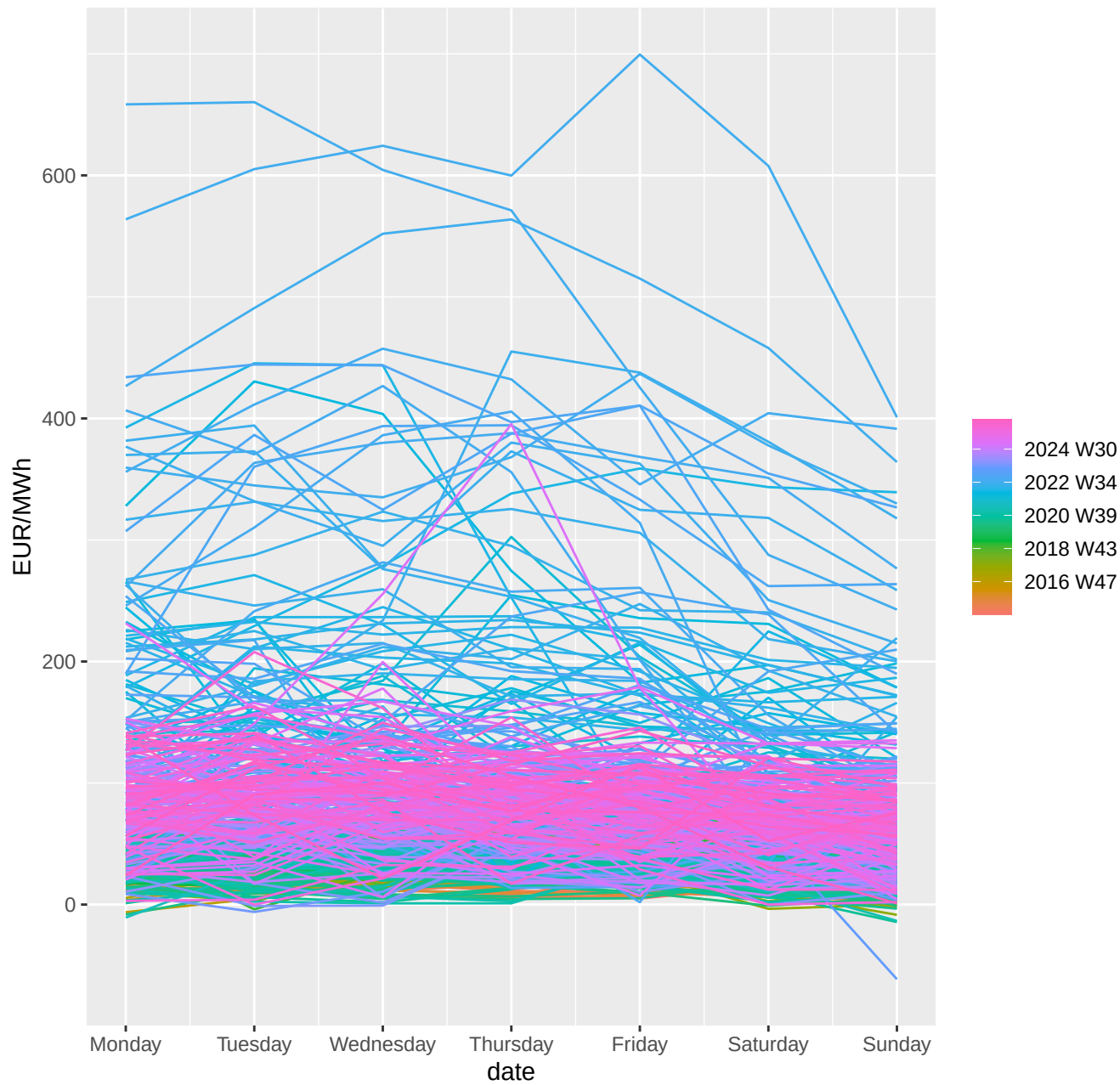
Weekly seasonality of DK1 prices
